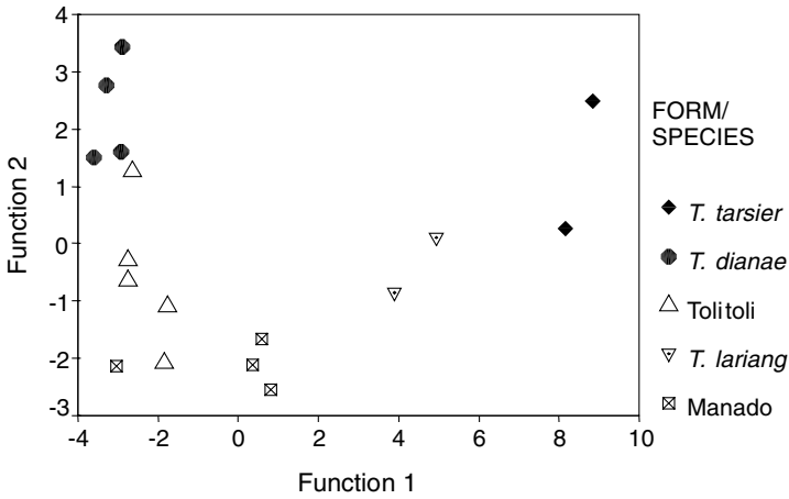
Fig. 8. Discriminant analysis of Sulawesi tarsiers based on 6 external measurements. The weightings of the original variables on the first discriminant function, which accounts for 76% of the total variation, are as follows: Head + body length = -0.193, Tail length = -0.880, Hindfoot length = -0.509, 3rd finger length = 0.915, 3rd finger pad length = 0.857, 3rd finger pad breadth = 0.881, 3rd finger nail length = 0.538, 3rd finger nail breadth = -0.432.
