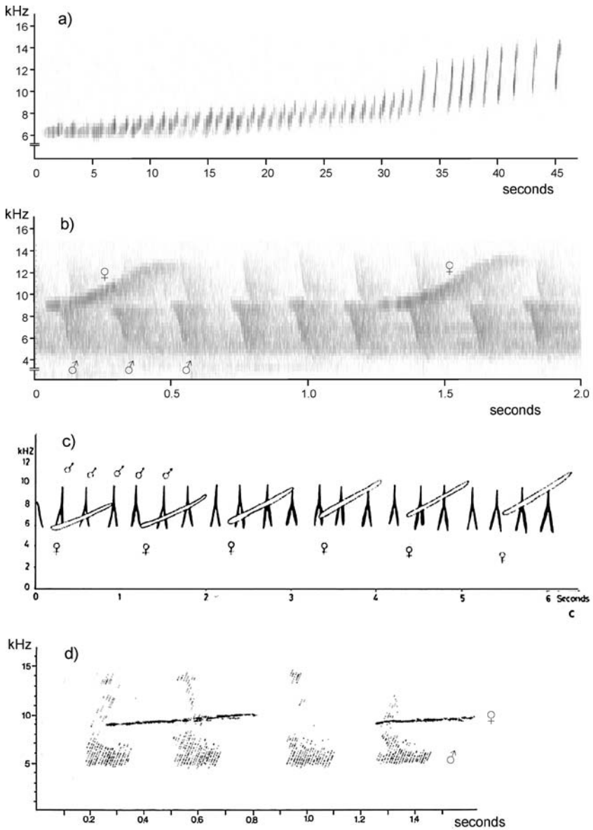
Fig. 10. Spectrograms of vocal duets of Tarsius larium . (a) Complete female part of a duet song. (b) Male and female notes at the end of a duet. (c) Fragment of a duet song (redrawn from MacKinnon and MacKinnon, 1980). (d) Fragment of a duet song (redrawn from Niemitz 1984b).
