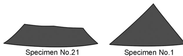
Fig. 3. Examples of the range of flake cross-sections used in the reduction experiment. Specimen No. 21 has a flattish trapezoidal-like cross-section similar to Dibble’s “flat flakes”, while Specimen No. 1 has a steep triangular cross-section.
