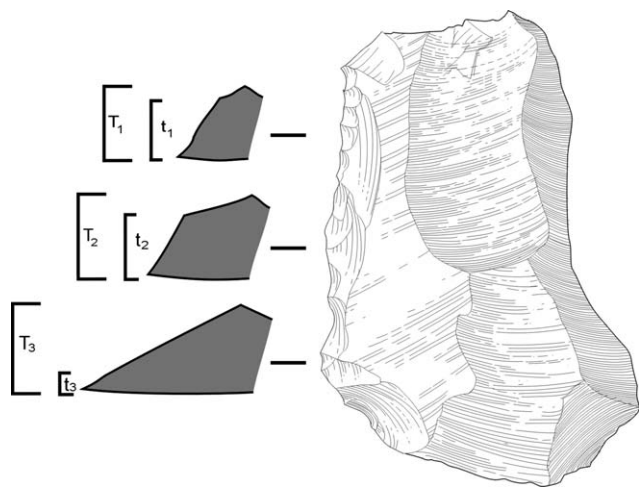
Fig. 1. Illustration of the measurement of Kuhn's [19] Geometric Index of reduction on a uniaxially retouched flake.
